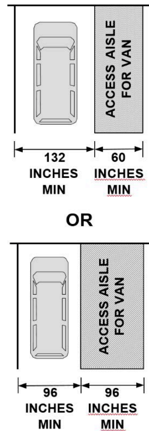
Figure 2: Access aisle
